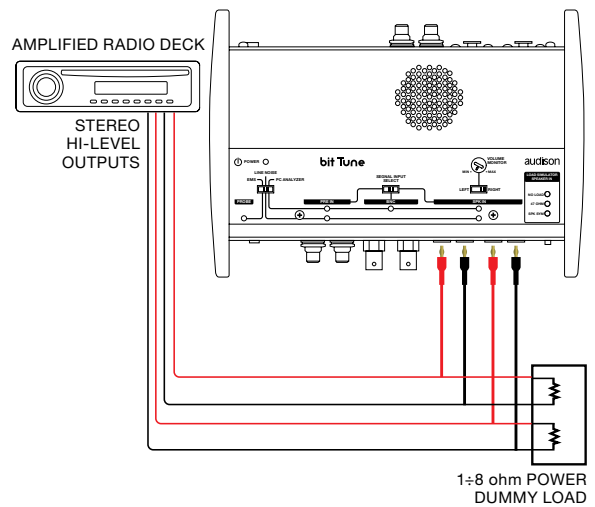
4. SPEAKER IN: HEAD UNIT POWER ANALYZER (see sect. 7.1 - 8.3)
