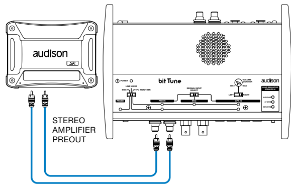
2. PRE IN: AMPLIFIER PREOUT ANALYZER (see sect. 7.1 - 8.3)
