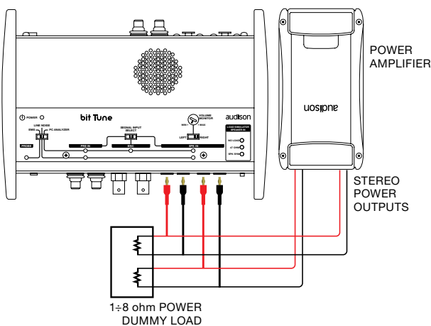
5. SPEAKER IN: AMPLIFIER POWER ANALYZER (see sect. 7.10)
