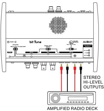
3. SPEAKER IN: HEAD UNIT HI LEVEL ANALYZER (see sect. 7.1 - 8.3)
