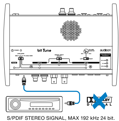
6. OPTICAL IN: HEAD UNIT OPTICAL TEST (see sect. 8.3)
