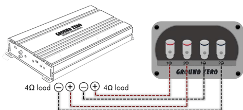
stereo wiring @ 4Ω load/channel
