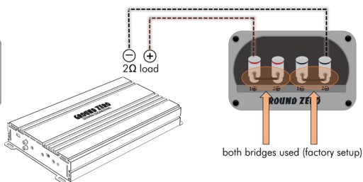
Parallel wiring with one mono amplifier @ 2Ω load
